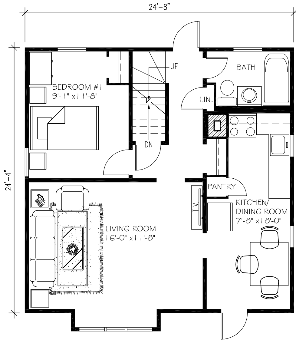
1 FIRST FLOOR PLAN SCALE 3/16" = 1'-0"
