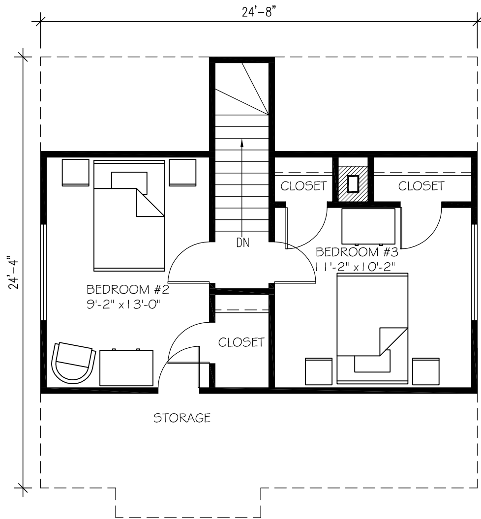
2 SECOND FLOOR PLAN SCALE 3/16" = 1'-0"
